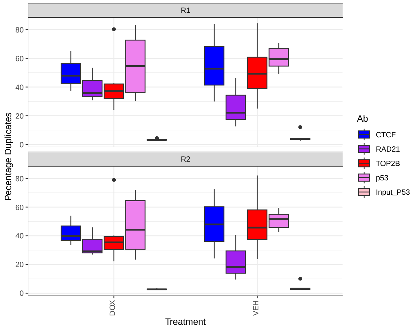
Percent duplication by sample, Merged Runs by Treatment
